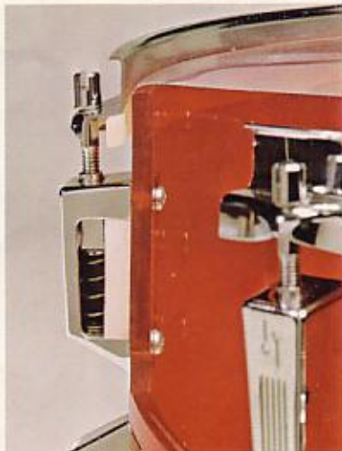
Self-aligning, spring-loaded inserts allow fast and easy tensioning of the heads.
